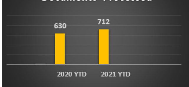
Documents Processed
