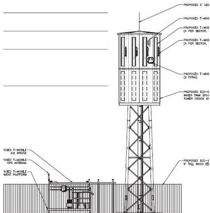
Figure 2: Proposed water tower design
