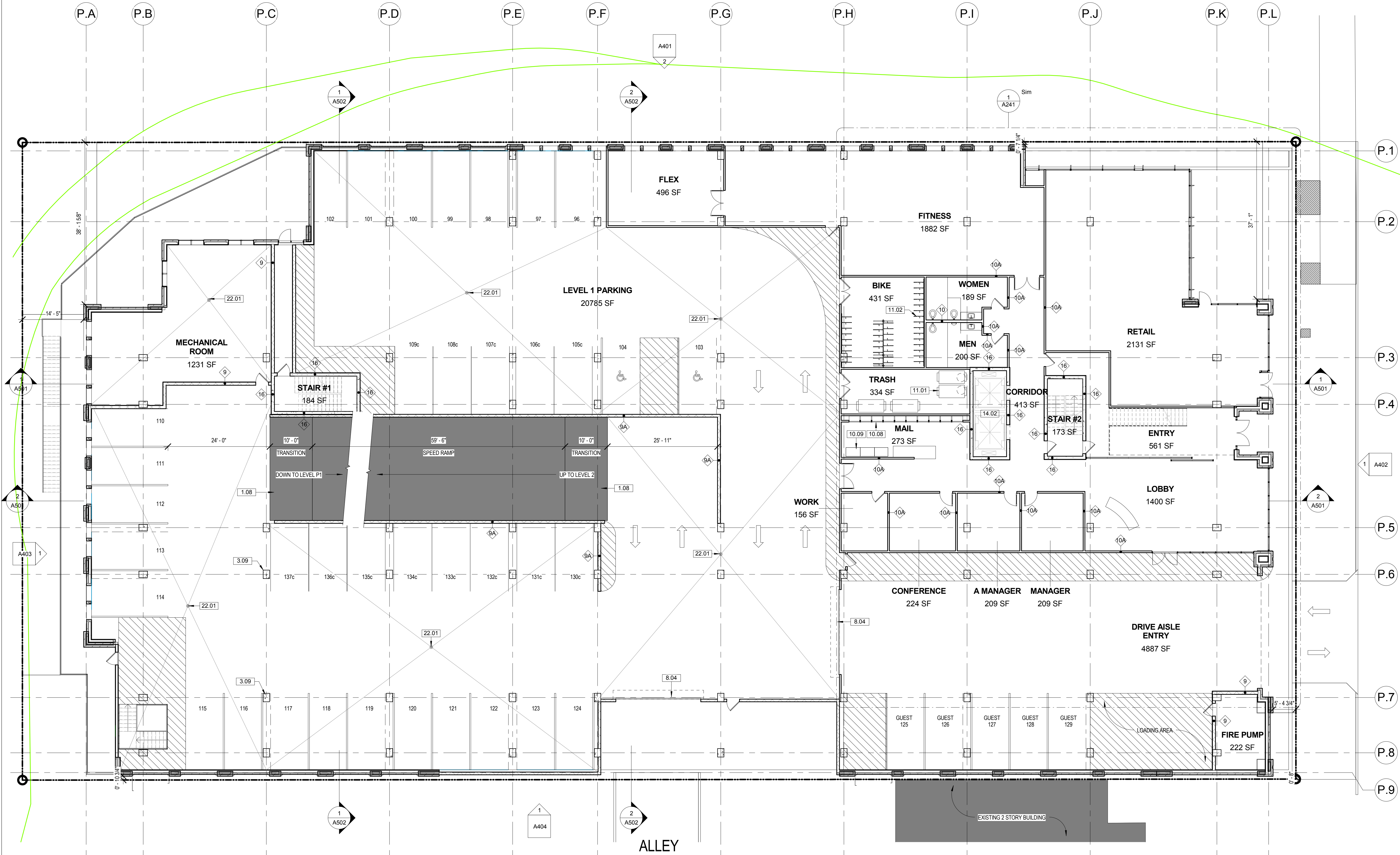
1 LEVEL 1 BUILDING PLAN 3/32" = 1'-0"
