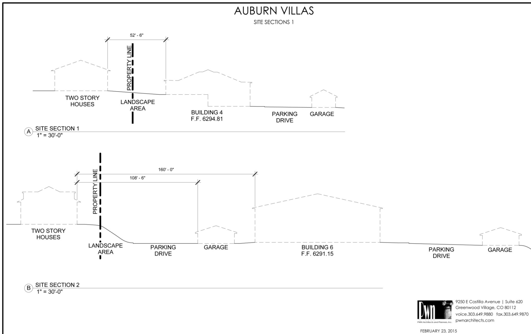
FIGURE 2 – SITE SECTIONS
