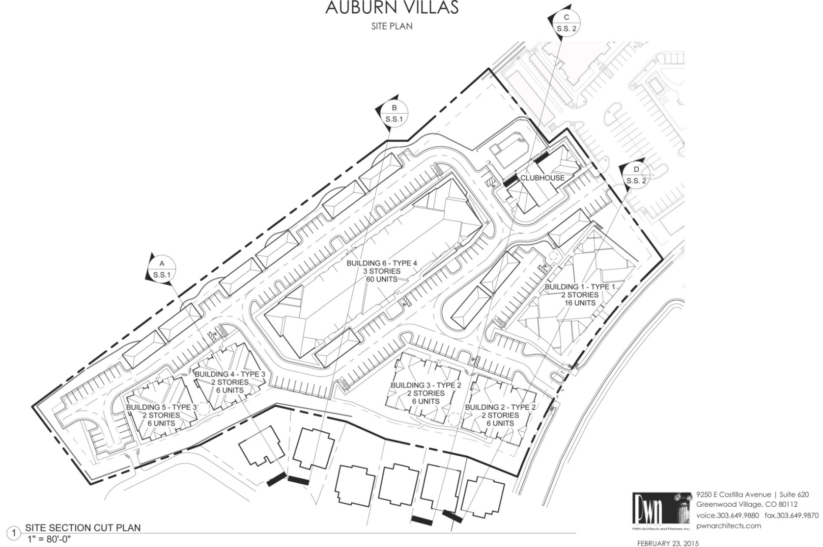
FIGURE 2 – SECTION CUT SITE PLAN
