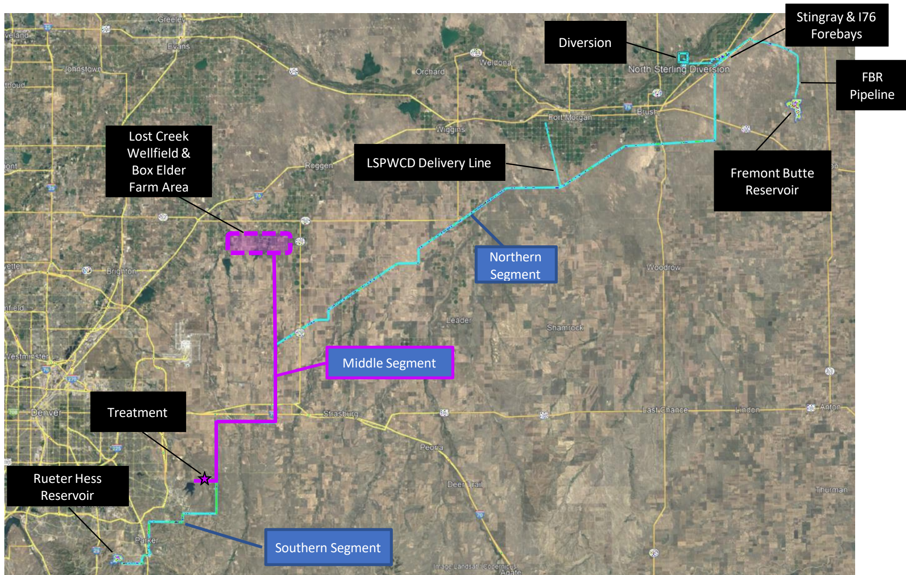
PVWP System
