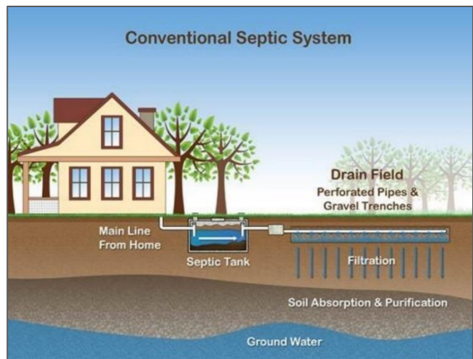
Figure 17: Conventional Septic System (Tri-County Health Department, 2016)
