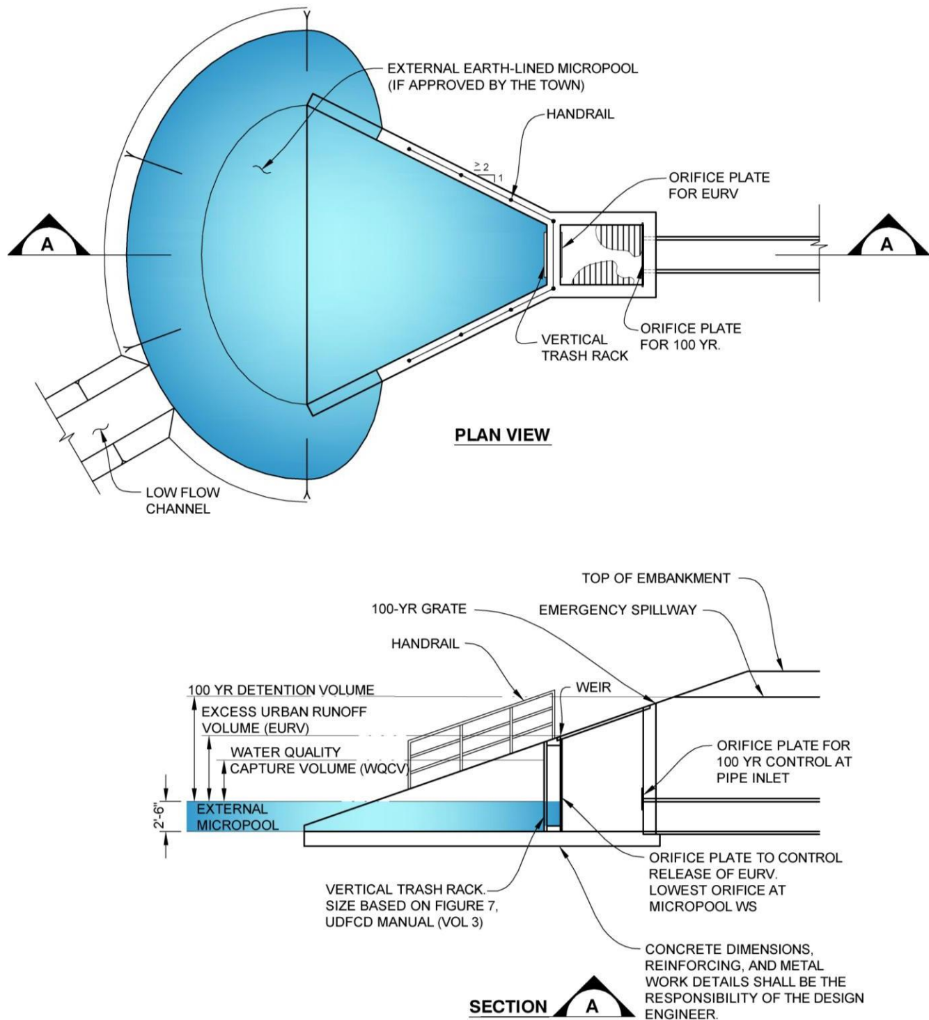
FIGURE 14-7 CONCEPT FOR OUTLET STRUCTURE WITH FLARED WINGWALLS AND HANDRAIL (EXTERNAL MICROPOOL SHOWN)
