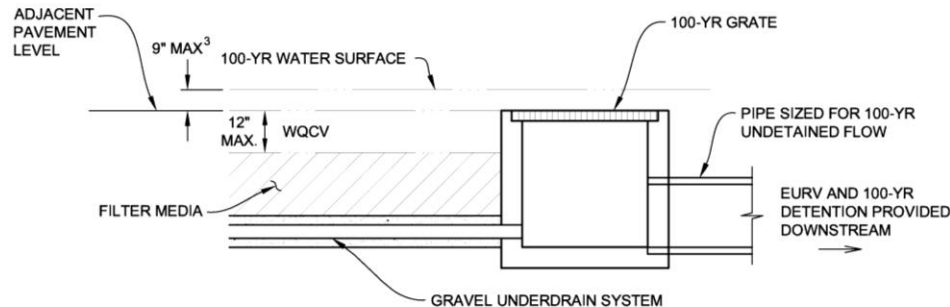
OUTLET STRUCTURE WHERE WQCV AND EURV ARE COMBINED; 100-YEAR DETENTION IS PROVIDED DOWNSTREAM
