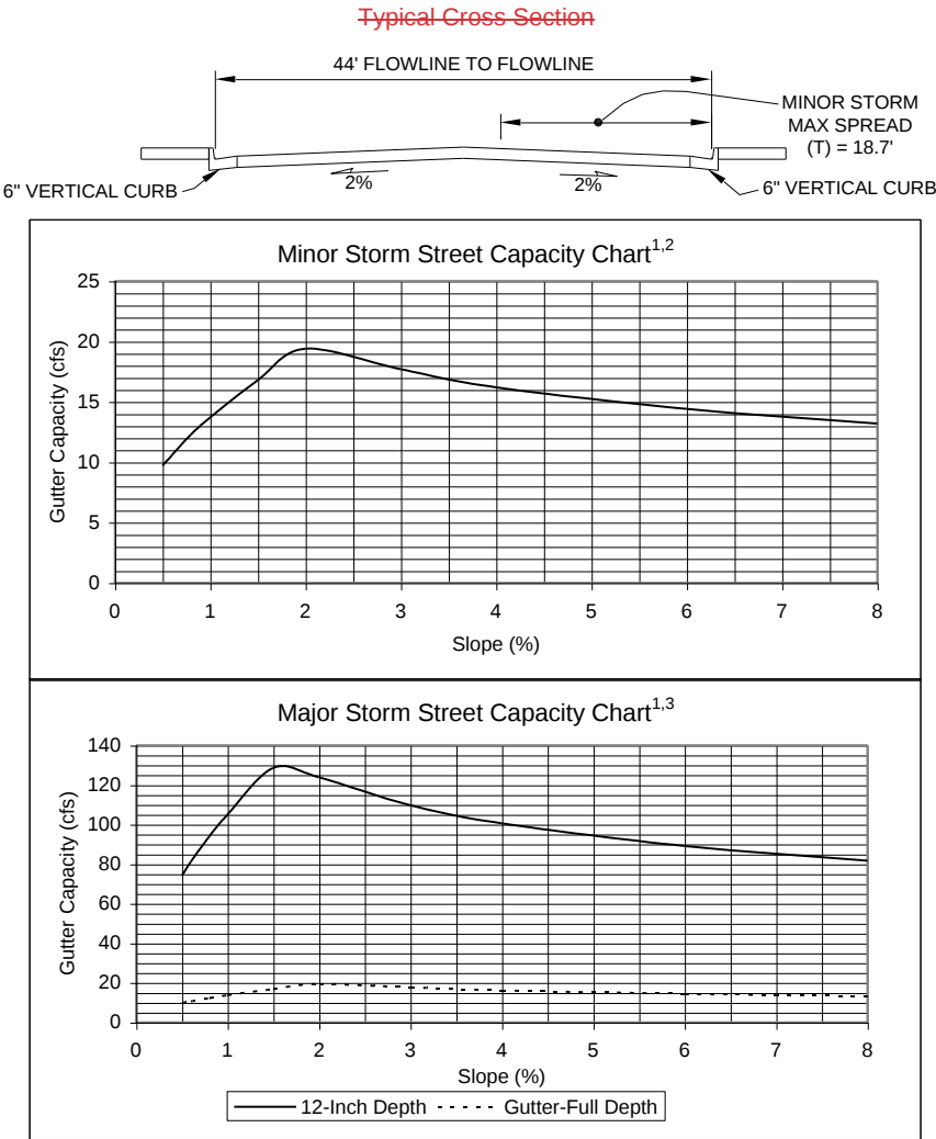
FIGURE 7-2, TOWN OF CASTLE ROCK STREET CAPACITY CHART LOCAL TYPE I AND TYPE II (MULTI-FAMILY)
