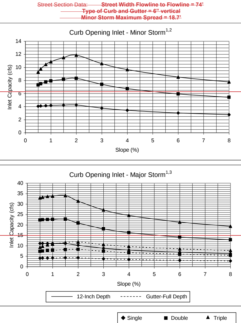
FIGURE 8-6, INLET CAPACITY CHART CURB OPENING (TYPE R) INLET MINOR ARTERIAL
