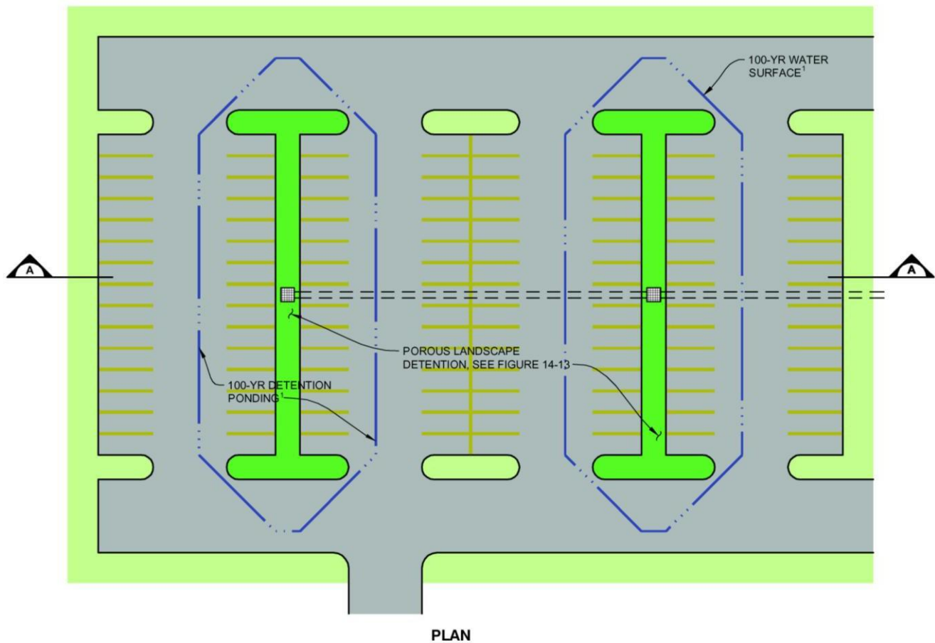
FIGURE 14-12 CONCEPT FOR POROUS LANDSCAPE DETENTION IN PARKING LOT
