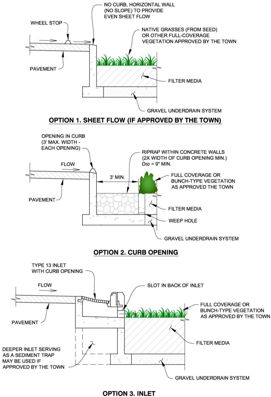
FIGURE 14-14 CONCEPTS FOR INFLOWS TO POROUS LANDSCAPE DETENTION IN PARKING LOT
