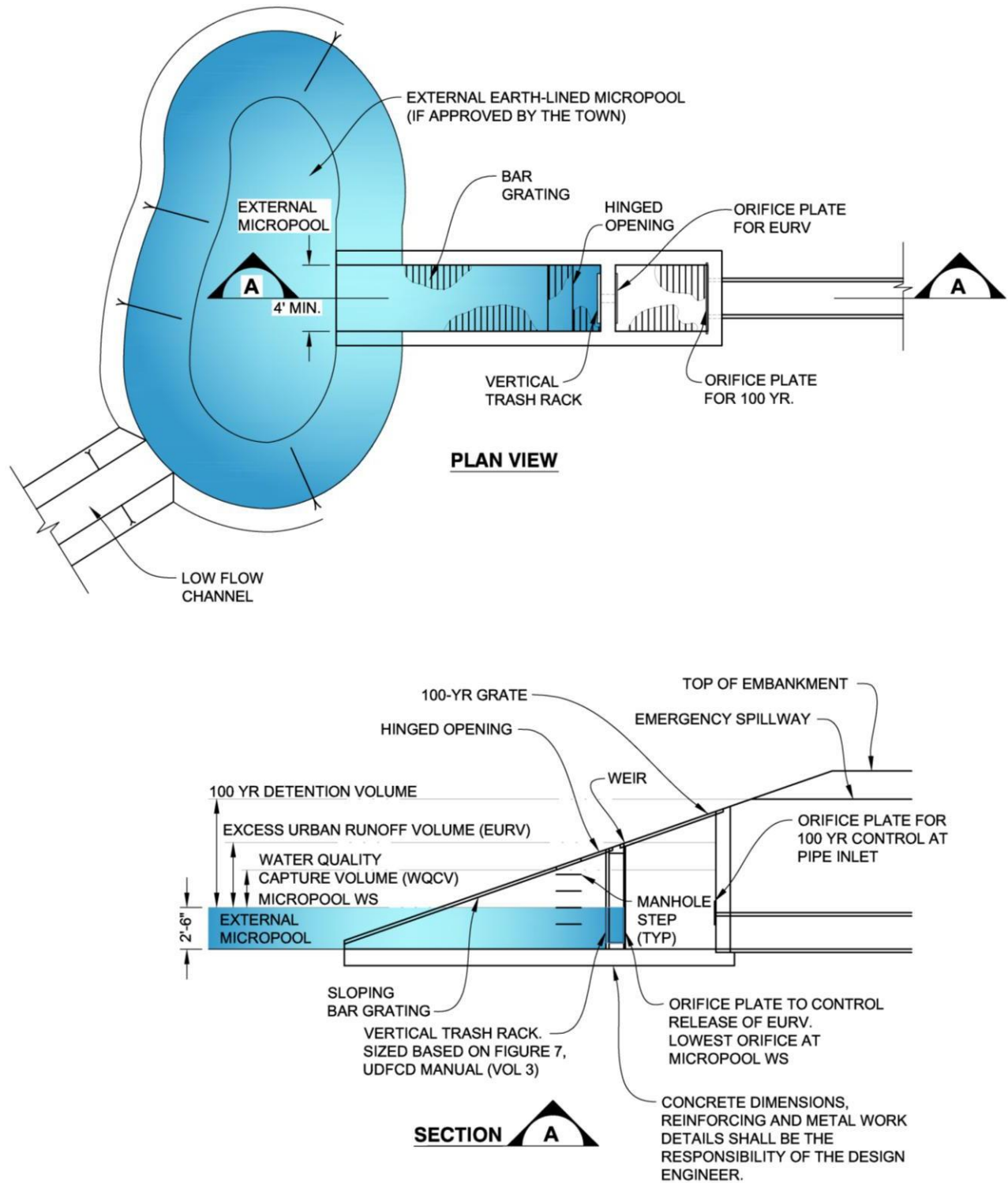
FIGURE 14-6 CONCEPT FOR OUTLET STRUCTURE WITH PARALLEL WINGWALLS AND FLUSH BAR GRATING (EXTERNAL MICROPOOL SHOWN)
