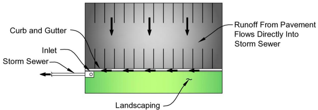
FIGURE 14-1 TERMS FOR MINIMIZING DIRECTLY CONNECTED IMPERVIOUS AREA
