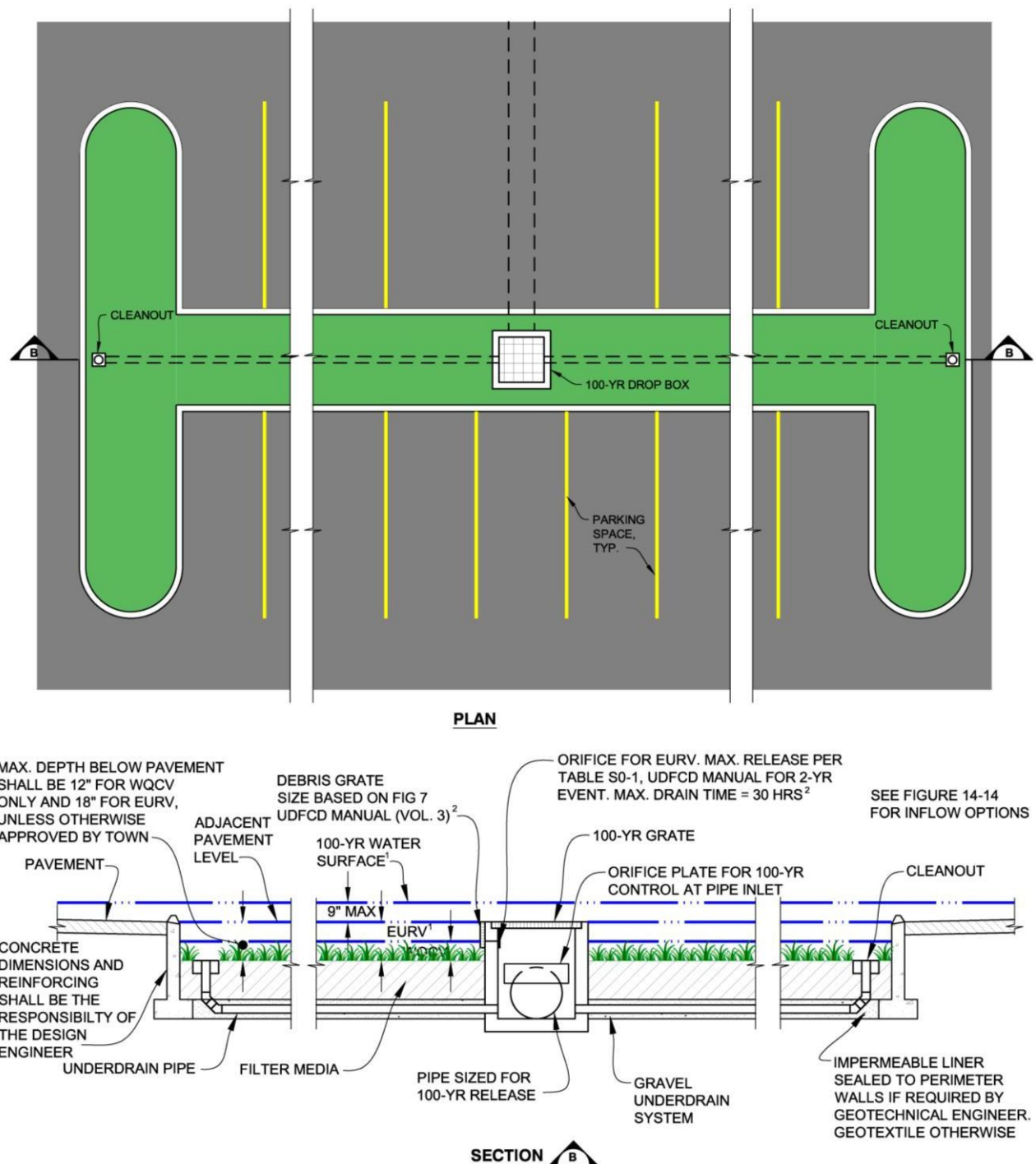
FIGURE 14-13 CONCEPT FOR POROUS LANDSCAPE DETENTION IN PARKING LOT (DETAILED VIEW)
