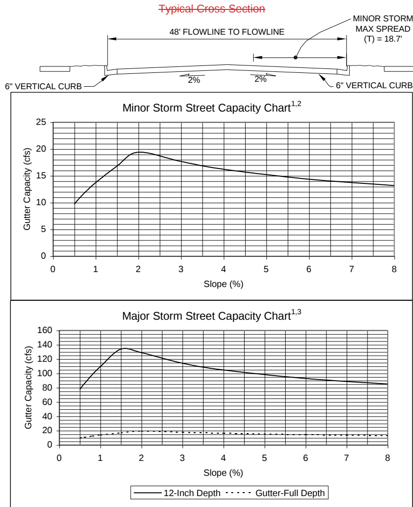
FIGURE 7-4, TOWN OF CASTLE ROCK STREET CAPACITY CHART MINOR COLLECTOR
