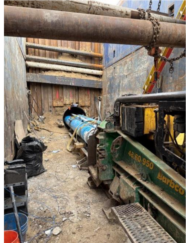
DIA Connection pipeline bore under E-470
