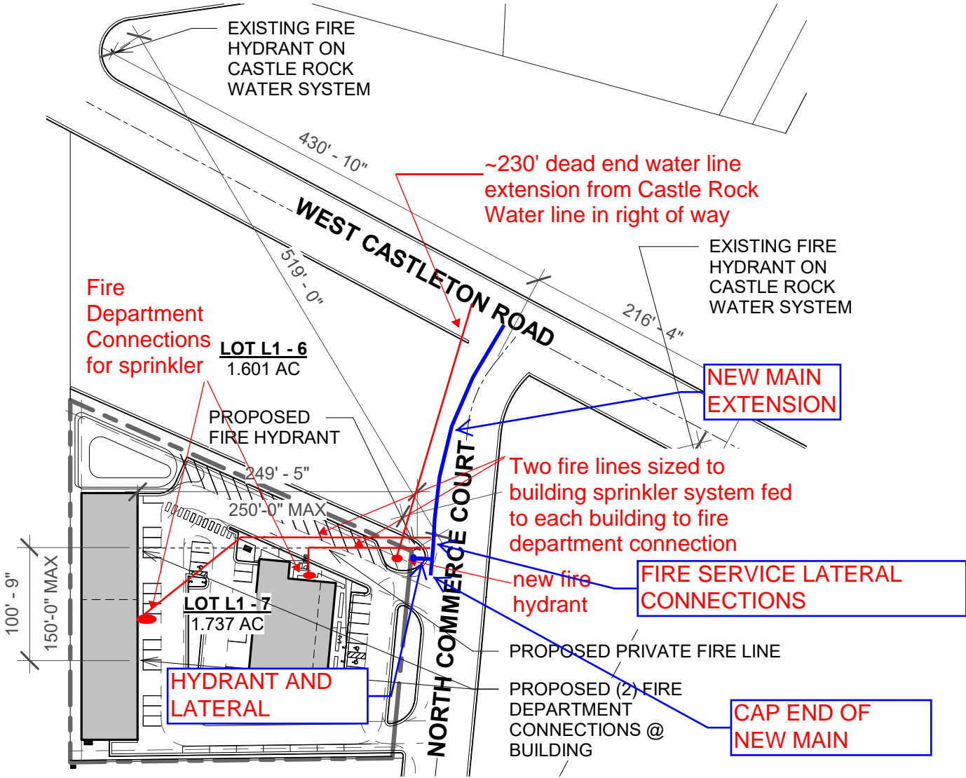
VICINITY MAP - FIRE HYDRANT LOCATIONS
