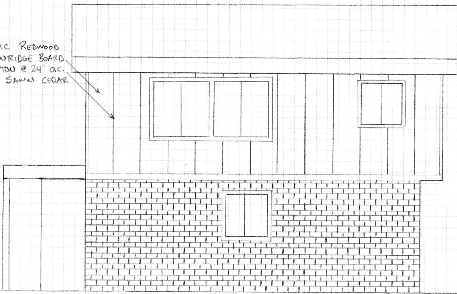
SIDE ELEVATION
