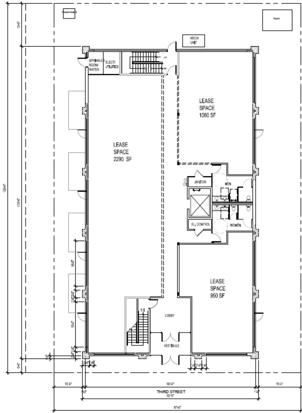
1 PLAN 1st FLOOR (2nd FLOOR SIM) A2.0 SCALE: 1" = 3/32"
