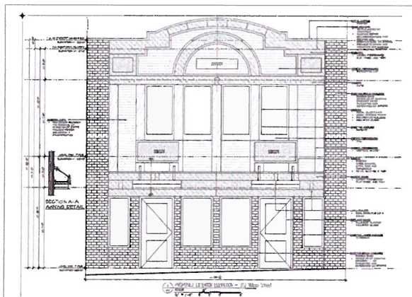
Proposed Elevation
