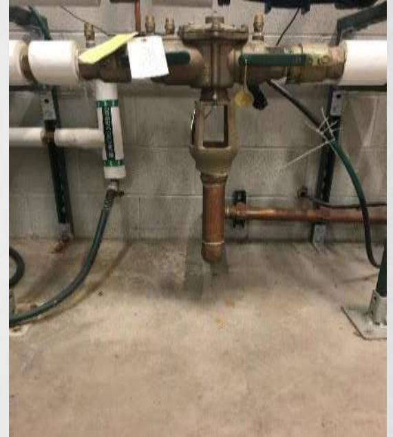
Reduced Pressure Zone Assembly Commercial Application
