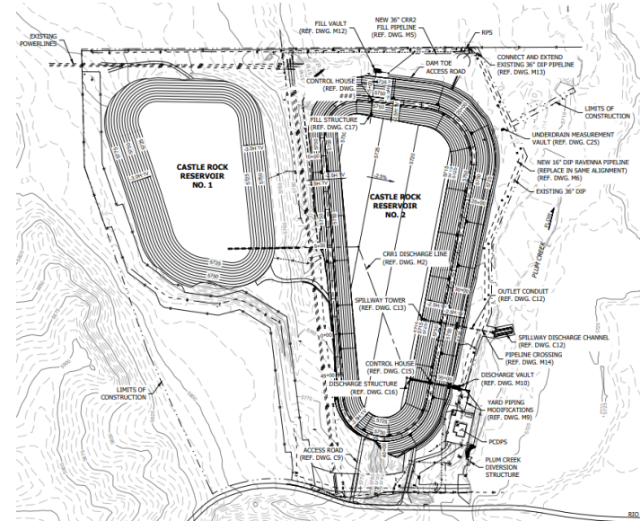
CRR1 and CRR2 Final Designs
