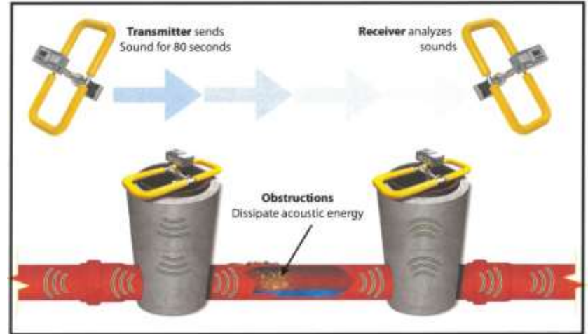
Sewer Line Assessment Process
