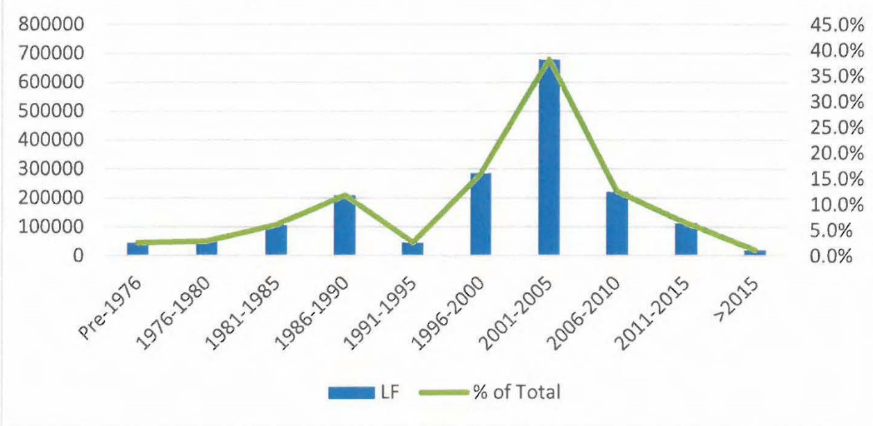
Fig 3.2 Potable Water Main Age
