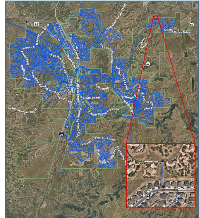
Location of the Castle Rock – Pinery water system interconnect
