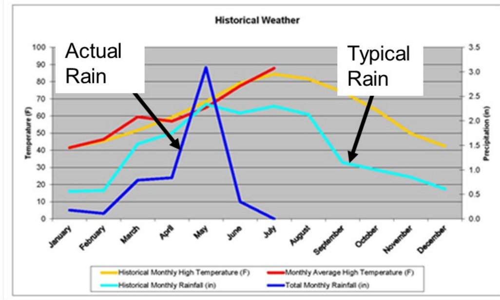
Figure 2: 2017 Observed Temperatures and Precipitation as of July
