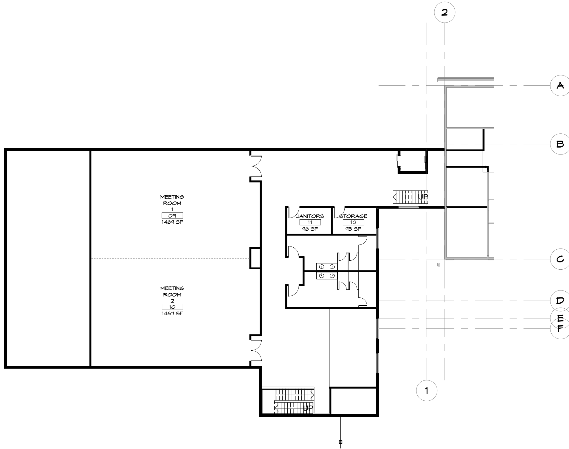
① OPTION 3 2ND FLOOR 1/16" = 1'-0"
